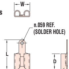
Non-Insulation Support Terminals (Solder)
