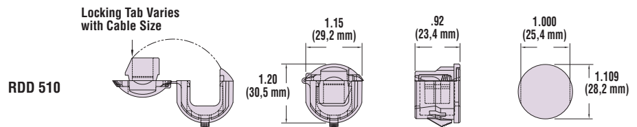
MOUNTING HOLE
