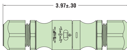
ASSEMBLED VIEW
