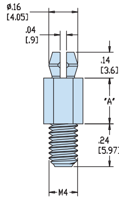
TWO PRONG SNAP FIT / M4 MALE THREAD
