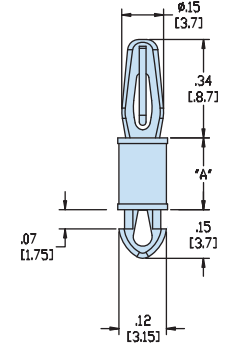
BAYONET SNAP LOCK 8,7 / TEARDROP SNAP LOCK
