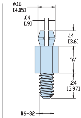
TWO PRONG SNAP FIT / 6-32 MALE THREAD
