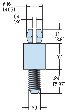
TWO PRONG SNAP FIT / M3 MALE THREAD
