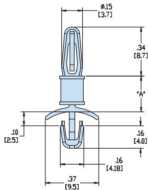
BAYONET SNAP LOCK 8,7 / ARROWHEAD SNAP LOCK
