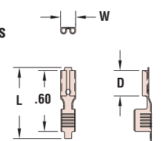
Non-Insulation Support Terminals (Crimp)
